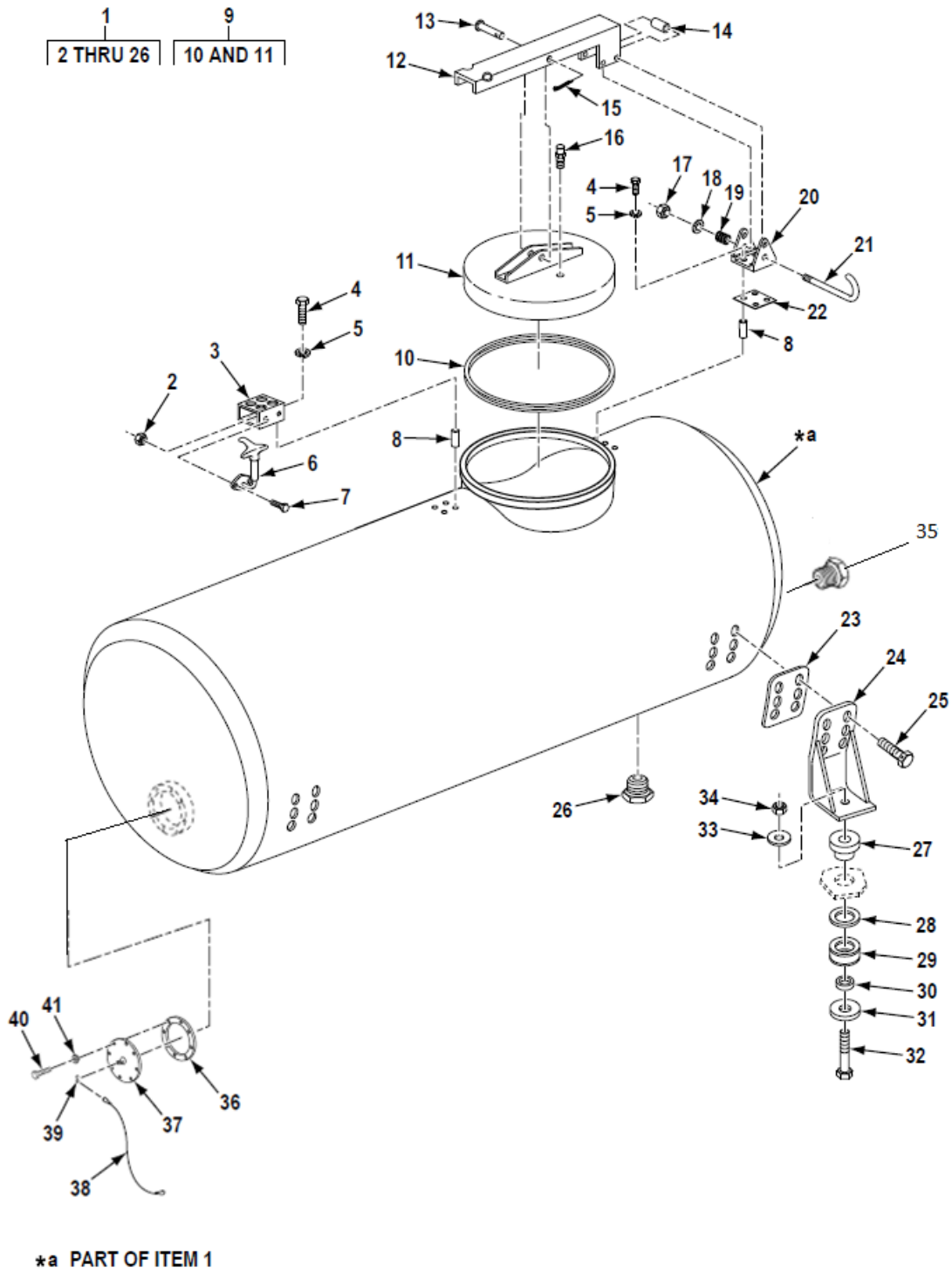
Figure 21. Water Tank, Body Brackets, and Manhole Cover.
