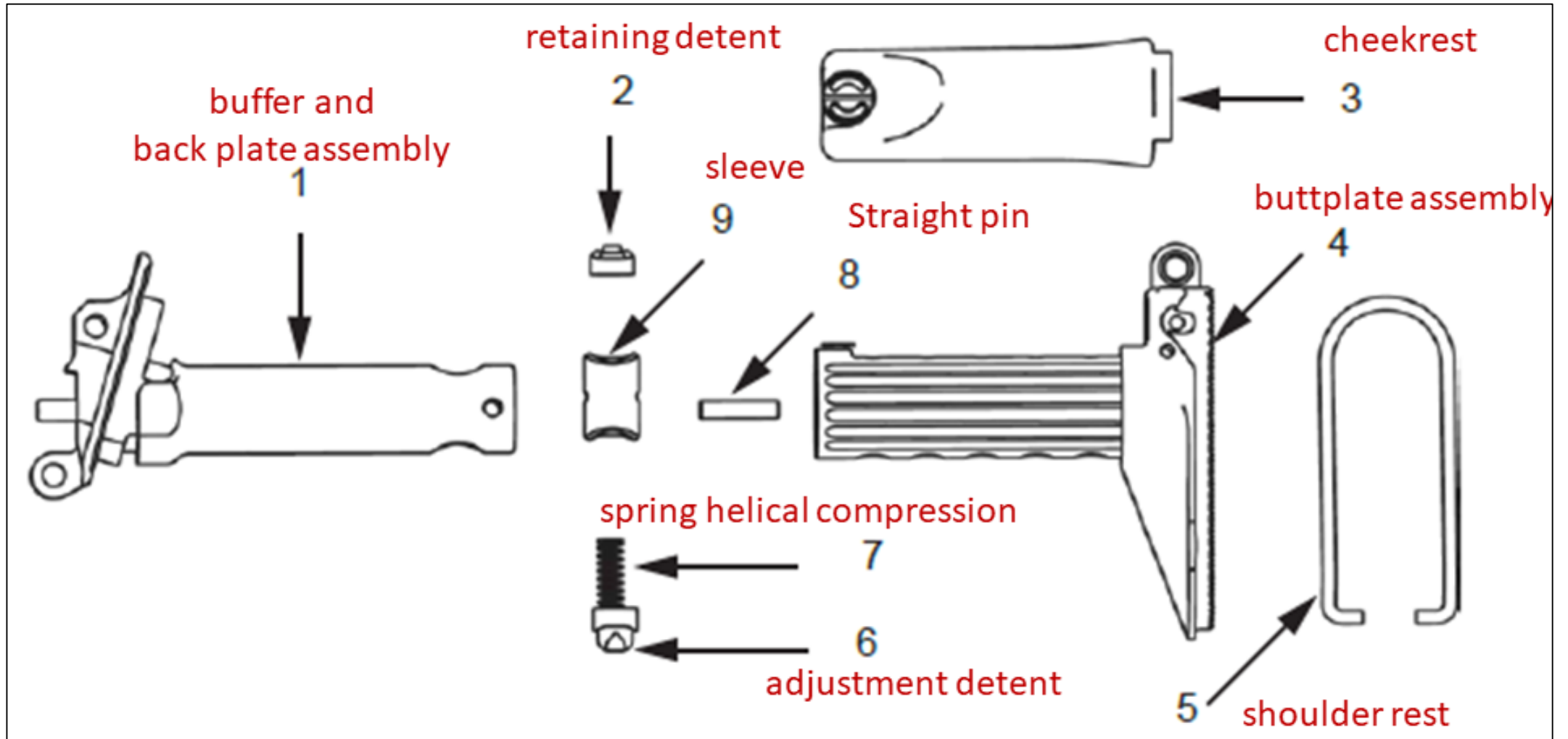
Fig 4. Lightweight collapsible buttstock disassembly
