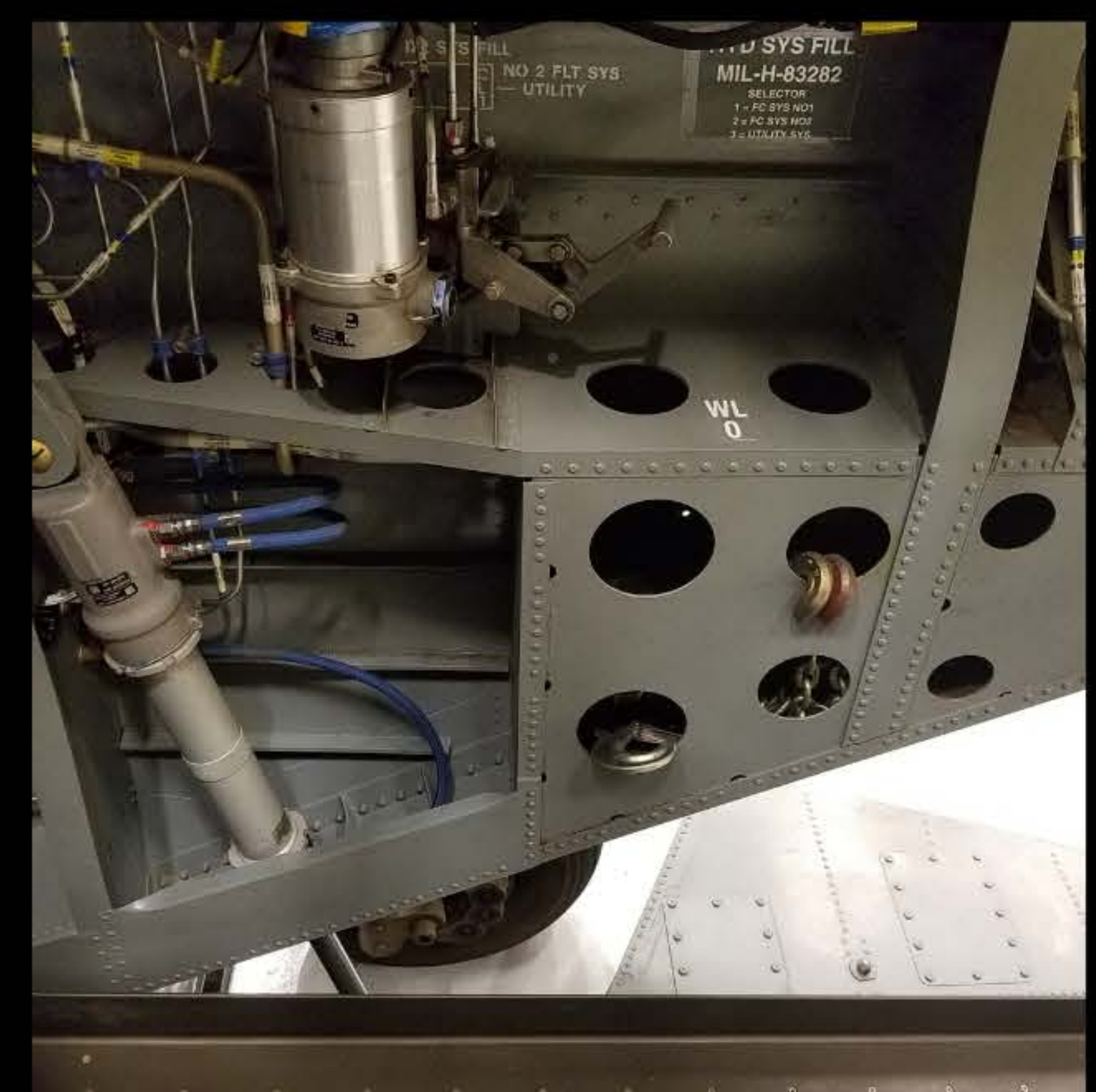
Don't store tie-down chains in canted beam area on either side of aircraft
